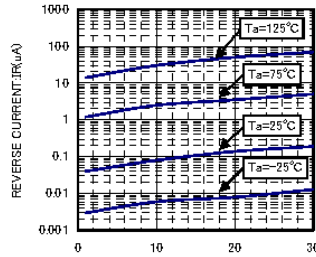
VR-IR CHARACTERISTICS
