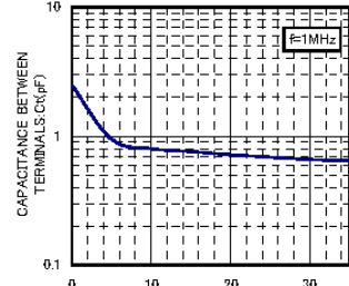
VR-Ct CHARACTERISTICS
