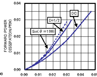
Io-PF CHARACTERISTICS
