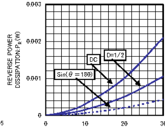
VR-Pk CHARACTERISTICS
